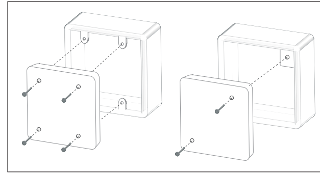
Fig 3. Mounting the FB-AP Series Switch Monitors (7254-FBD-5830)
