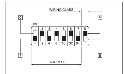
Fig 4. DIL Switch
