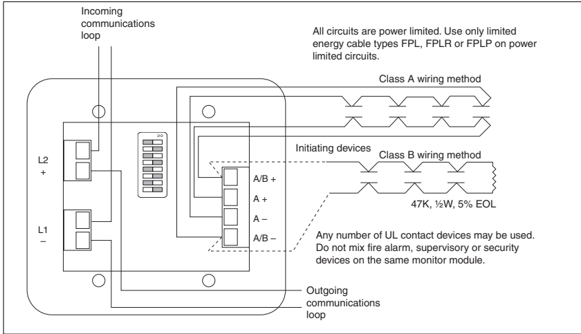
Fig 1. Wiring Diagram for FB-AP Series Priority Switch Monitor Module
